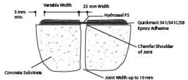
Construction Joints
